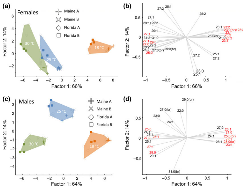
Fig. 4 Projection of principal component analysis (PCA) factor scores and variable correlations with the first two PCA factors, showing the quantitative patterns of cuticular hydrocarbons (CHCs) in female (a, b) and male (c, d) populations from two geographical regions (Florida and Maine) cultured at three different temperatures (18 °C, 25 °C and 30 °C). Variables in red were retrieved as among the most correlated with the Canonical Correspondence Analysis model using temperature as a categorical predictor. Longer-chain CHCs are strongly associated with the shift from lower to higher temperatures. For both sexes, longer-chain CHCs were observed to increase in abundance with increasing temperature.
