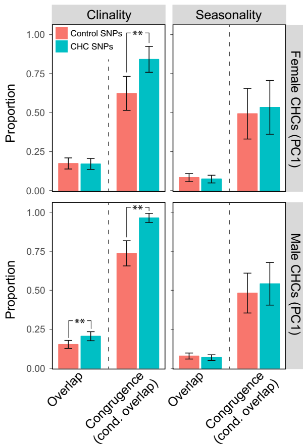
Fig. 7 Patterns of clinal and seasonal variation at SNPs associated with cuticular hydrocarbon (CHC) profiles and their genomic controls. Examination of overlap is based on co-occurrence of CHC SNPs among SNPs previously identified as clinal or seasonal (see Materials and Methods for details). Congruence of the direction of SNP effect in a genomewide association study was examined at SNPs that were both significantly associated with CHC PC1 and varied through time or space. ** corresponds to bootstrap P -value <0.01 .
