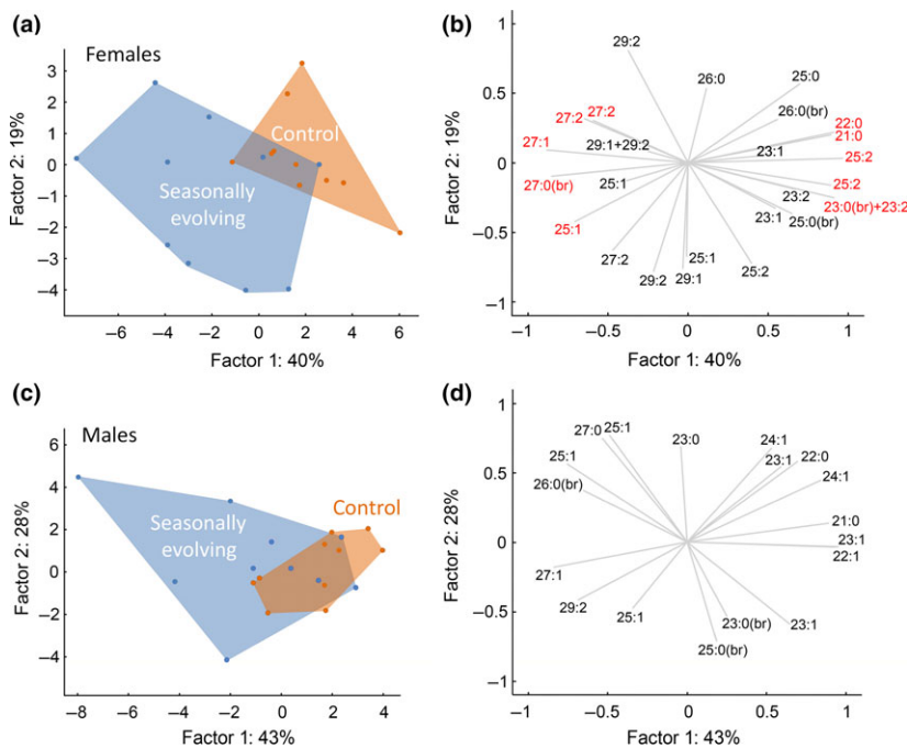
Fig. 6 Projection of principal component analysis (PCA) factor scores and variable correlations with the first two PCA factors of the quantitative patterns of cuticular hydrocarbons (CHCs) in control and evolving populations of females (a, b) and males (c, d). The visual representation suggested a differentiation between the experimental treatments, even though the two groups were slightly overlapping; the treatments differed significantly in CHC profiles for females only. The CHC profiles of the control, laboratory populations were more homogeneous in comparison with the seasonally evolving populations. Variables in red were retrieved as among the most correlated with the Canonical Correspondence Analysis model using treatment as a categorical predictor.
