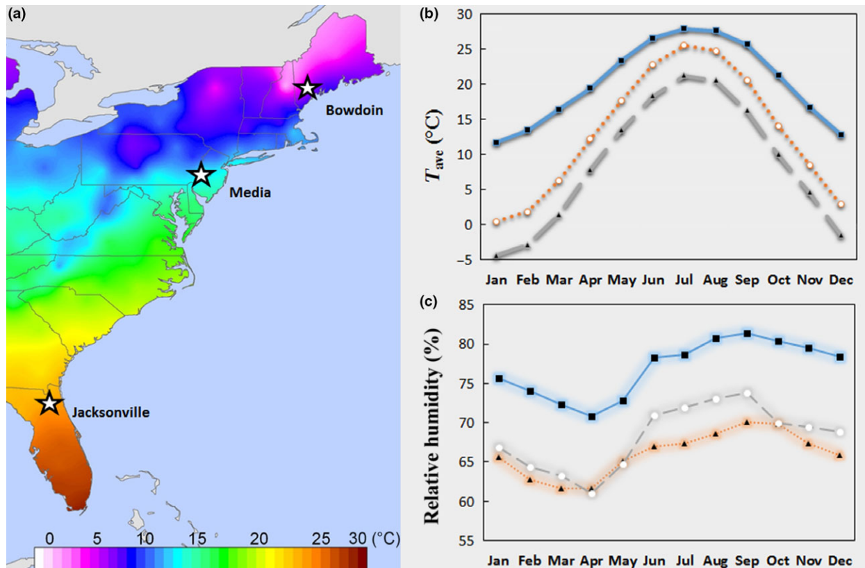
Fig. 1 Temperature map of the east coast of the United States of America (a). The three collection sites for natural Drosophila melanogaster populations are denoted by stars (Jacksonville, FL, 30.33°N, 81.66°W; Media, PA, 40.04°N, 76.30°W; Bowdoin, ME, 44.03°N, 73.20°W). Seasonal collections were made in the spring and fall in two successive years (2012 and 2013) from the Media, PA population. Thermal plasticity experiments were performed on FL and ME populations only. Twelve months' average temperature (b) and relative humidity (c) patterns for the sites of origin of populations. Jacksonville (30.33°N), Media (40.04°N) and Bowdoin (44.03°N) stations' T_{ave} and relative humidity are shown in solid (with rectangles), dotted (with circles) and dashed (with triangles) lines, respectively. Projections displayed here are the averages of 30 years (1980–2010). Climatic data were obtained from National Oceanic and Atmospheric Administration (NOAA; www.ncdc.noaa.gov).
