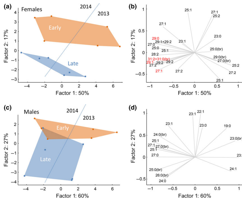
Fig. 5 Projection of principal component analysis (PCA) factor scores and variable correlations with the first two PCA factors, showing the quantitative patterns of cuticular hydrocarbons (CHCs) in female (a, b) and male (c, d) in populations from different years (2013 and 2014) and seasons (early (spring) and late (autumn)). When the year of collection was set as a categorical predictor in the Canonical Correspondence Analysis (CCA), a significant difference between 2013 and 2014 samples was observed. When the season was selected as a categorical predictor, significant differences were observed between early and late season samples in females, in which CHCs with relatively longer chain lengths were more represented in the late season collections. Variables in red were retrieved as among the most correlated with the CCA model using the season as a categorical predictor.
