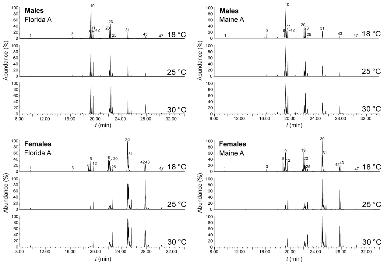
Fig. 2 Representative GC chromatograms showing cuticular hydrocarbons (CHCs) of males and females from two different localities (FL and ME) and cultured at three different temperatures. Note the shift towards longer-chain CHCs with the increasing temperature. Peak identifications: 1: n -heptacosane; 3: n -heneicosane; 6: ( Z,Z )-7,11-tricosadiene; 8: ( Z )-9-tricosene; 9: ( Z )-7-tricosene; 10: ( Z )-7-tricosene; 11: ( Z )-5-tricosene; 12: n -tricosane; 19: ( Z,Z )-7,11-pentacosadiene; 20: 2-methyltetracosane; 23: ( Z )-7-pentacosene; 25: n -pentacosane; 30: ( Z,Z )-7,11-heptacosadiene; 31: 2-methylhexacosane; 42: ( Z,Z )-7,11-nonacosadiene; 43: 2-methyloctacosane; 47: 2-methyltriacontane + hentriacontadiene. For other peaks, see Table 1.
