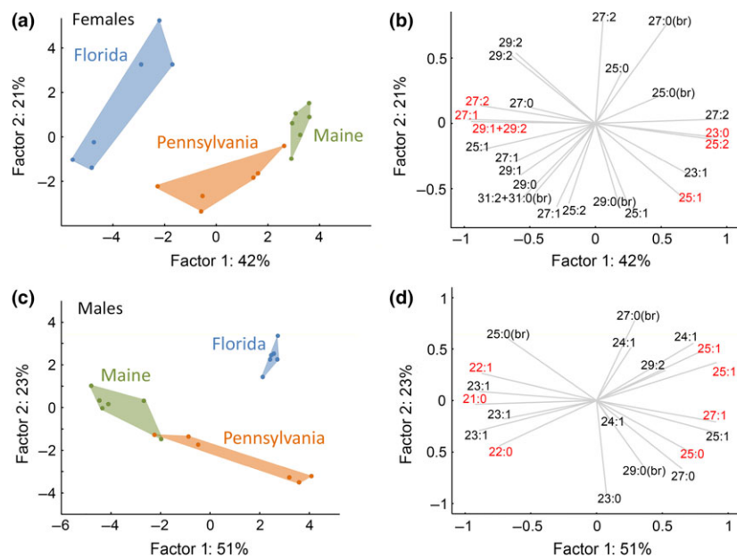
Fig. 3 Projection of principal component analysis (PCA) factor scores and variable correlations with the first two PCA factors of the quantitative patterns of cuticular hydrocarbons (CHCs) at 25 °C in females (a, b) and males (c, d) from the three geographically distinct populations. PCA clearly separated the populations (Florida, Pennsylvania and Maine) and for both sexes, the geographical differences were significant. In both sexes, the variables retrieved to have the best fit with the model predictions were longer-chain CHCs, over-represented in the Florida populations, whereas shorter-chain CHCs were more abundant in the remaining two populations (Pennsylvania and Maine). Variables in red were retrieved as among the most correlated with the Canonical Correspondence Analysis model using locality as a categorical predictor.
